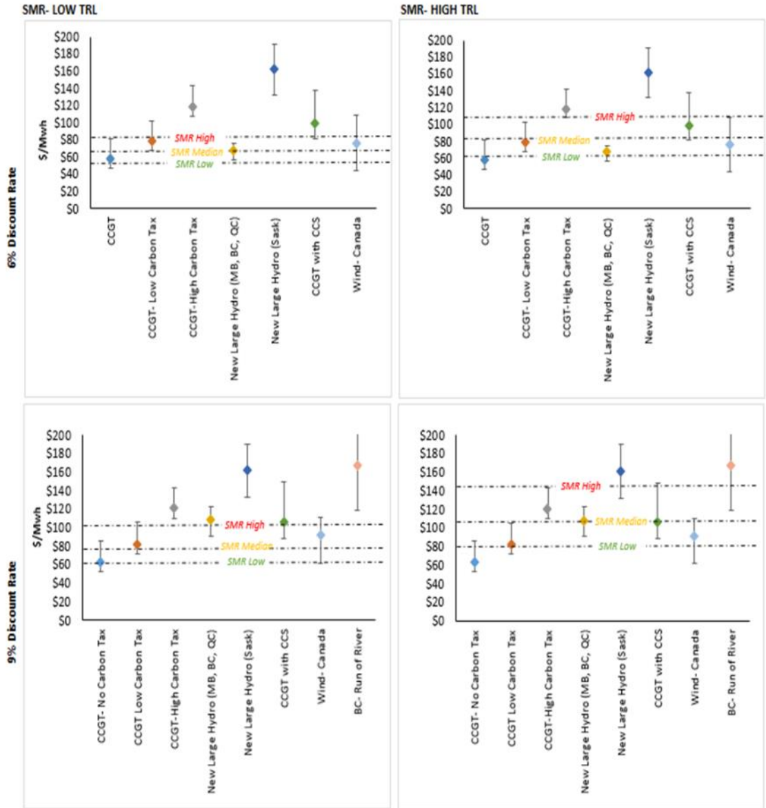
Figure 10 On-grid LCOE at 6% and 9% discount rates
